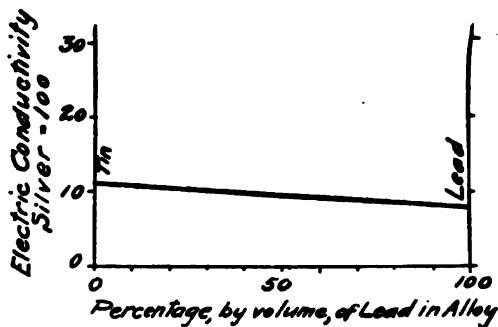
Fig. 55. Electric Conductivity Curve of the Lead-tin Alloys. Matthiessen, Rept. British Assoc. , XXXIII, p. 46, Pl. V, 1863.
